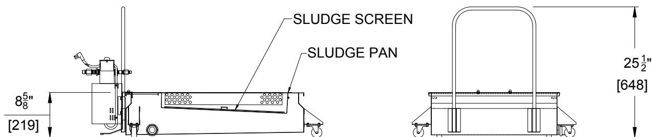
SIDE VIEW
