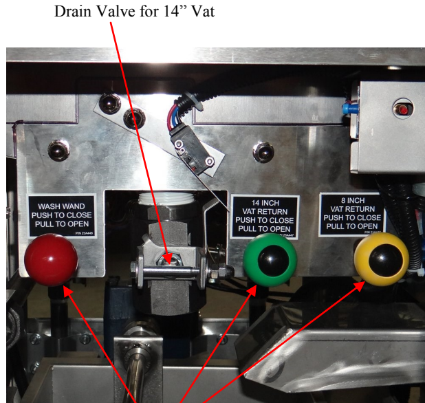
Push/Pull Levers
