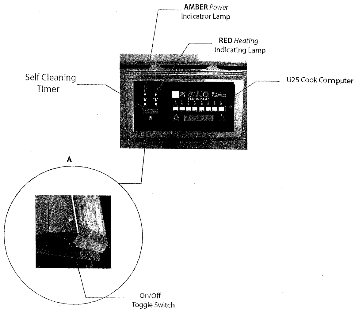
Figure1. PAR-3 Gas Fryer Components Location
